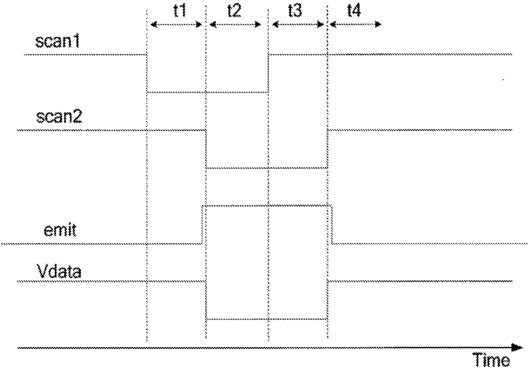
Fig. 2 (Prior Art)
